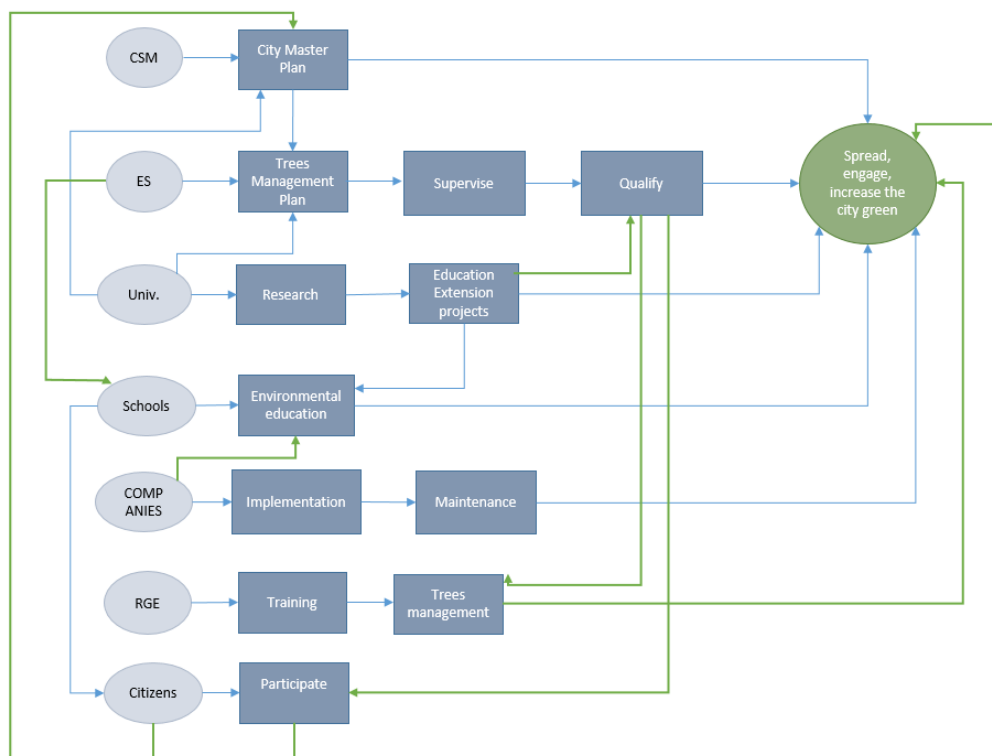
Figure 6. Proposed framework.
