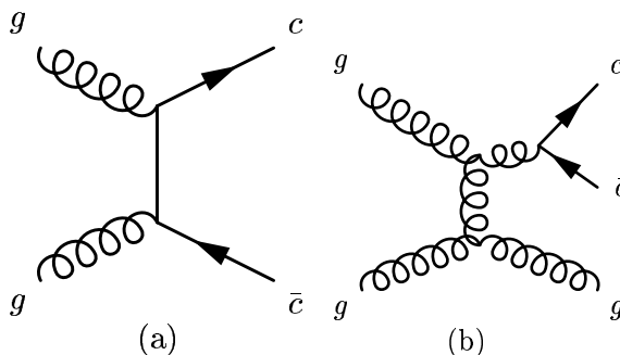
Figure 1: Illustration of c\bar{c} production processes in (a) leading order ( \alpha_s^2 ) and (b) next-to-leading order ( \alpha_s^3 ).
