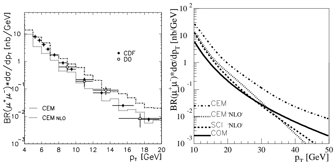
Figure 4: Distribution in transverse momentum of prompt J/\psi at (a) the Tevatron and (b) LHC ( |\eta| < 2.5 as for ATLAS) for the colour octet model (COM) based on NLO \mathcal{O}(\alpha_s^3) matrix elements (from [8]) and for the colour evaporation model (CEM) including g \rightarrow c\bar{c} to all orders in the parton shower and in the ‘NLO’ approximation where only c\bar{c} pairs from the first branching have been included. The result of this ‘first branching’ approximation applied to the soft colour interaction model (SCI) is also shown in (b).
