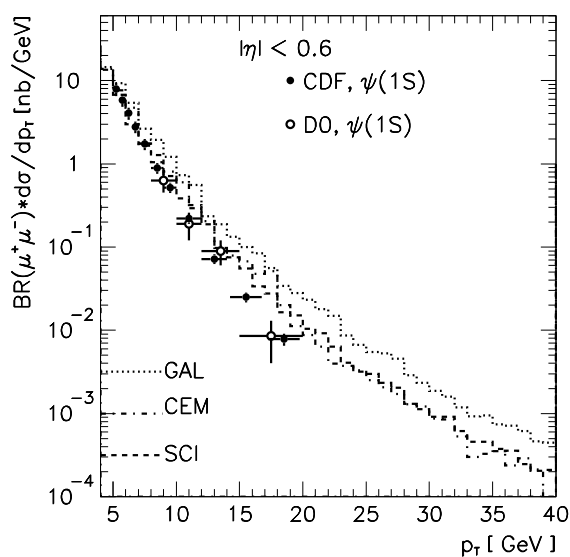
Figure 2: Distribution in transverse momentum of prompt J/\psi as observed by CDF and D0 [1] in p\bar{p} interactions at the Tevatron and obtained in the CEM, SCI and GAL models.
