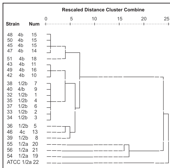
FIGURE 5 - Dendrogram of Listeria monocytogenes RAPD for strains isolated in southern Brazil and strains A51, A55 and ATCC 7,645, using the primer UBC 155 and serovar discrimination.
