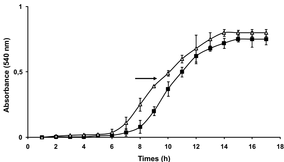
FIGURE 1 - Growth curve of B. pumilus ( \Delta ) and B. amyloliquefaciens ( \blacksquare ) on modified liquid Simmons medium at 28°C. The inflection point in the exponential growth phase was reached at 0.45 absorbance, as shown by the arrow. The inflection point was estimated according to the literature. Each data point indicates the mean growth of endophytic bacteria in three replications, and vertical bars represent the standard error of the means.
