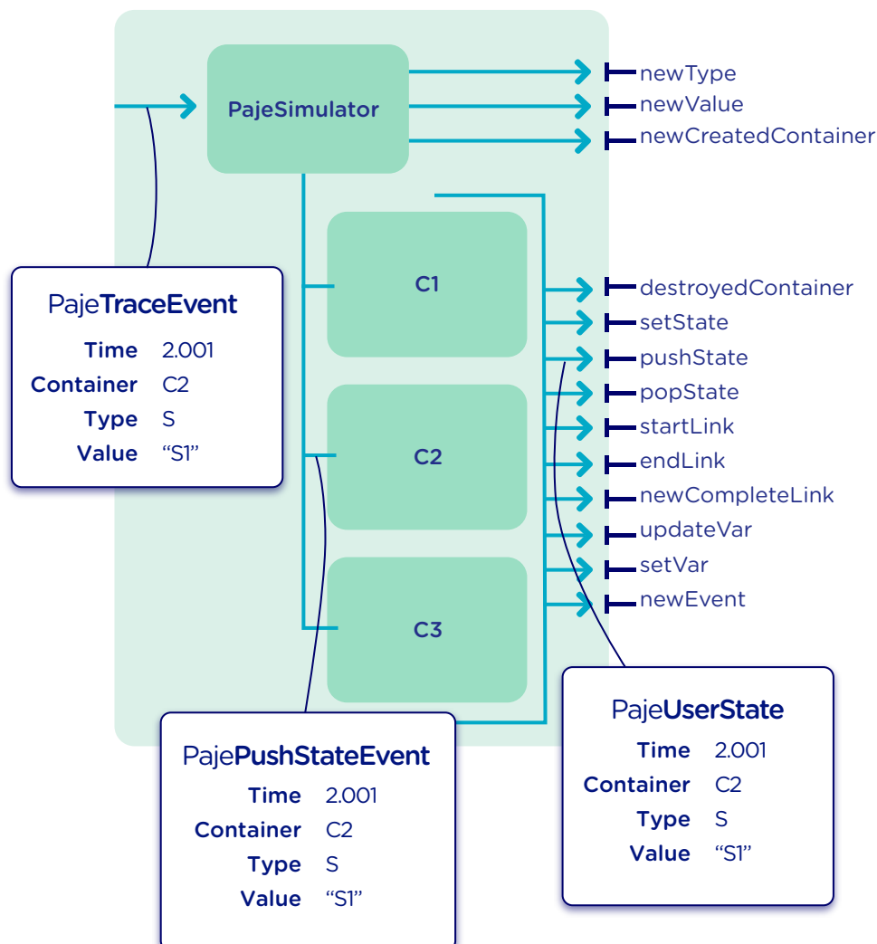
Figure 4.2: Aiyra's Core Architecture Core Simulator
