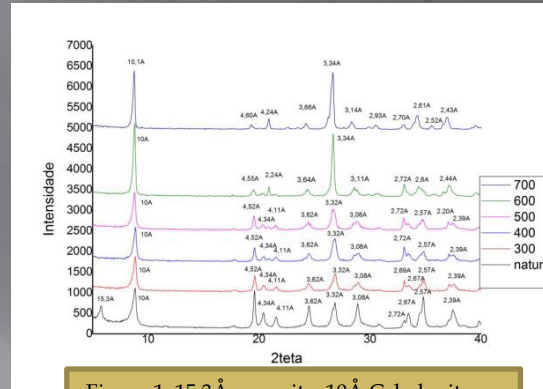
Figura 1: 15,3Å saponita; 10Å Celadonita; 10,1Å Fengita; 2,24Å Quartzo, 2,72Å Pirita;
