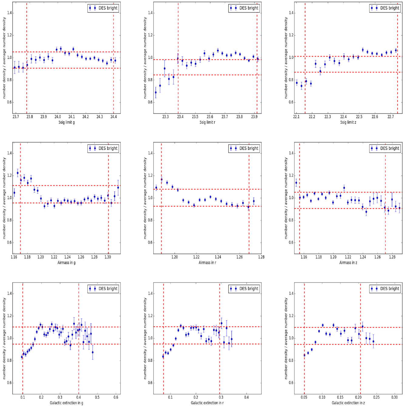
Figure D1. Density fluctuation of galaxies as a function of the depth, airmass and Galactic extinction in the top, middle and bottom row for the g,r,z bands. The two vertical and horizontal red axes show respectively the 5 and 95 per cent of the depth, airmass, galactic extinction distribution and 15 per cent around the mean galaxy density fluctuate ion for the eBOSS target selection.
