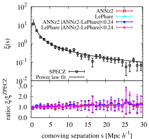
Figure 13. Comparison of \xi(s) for different redshift selections for the faint sample only. The top panel shows the monopole for the clean z_{\text{sp}} sample between 0.6 < z < 1.2 . The bottom panel shows the ratio between different redshift selections and the clean sample. An apparent increase on the clustering at large scales is seen for the photometric redshifts selections.
