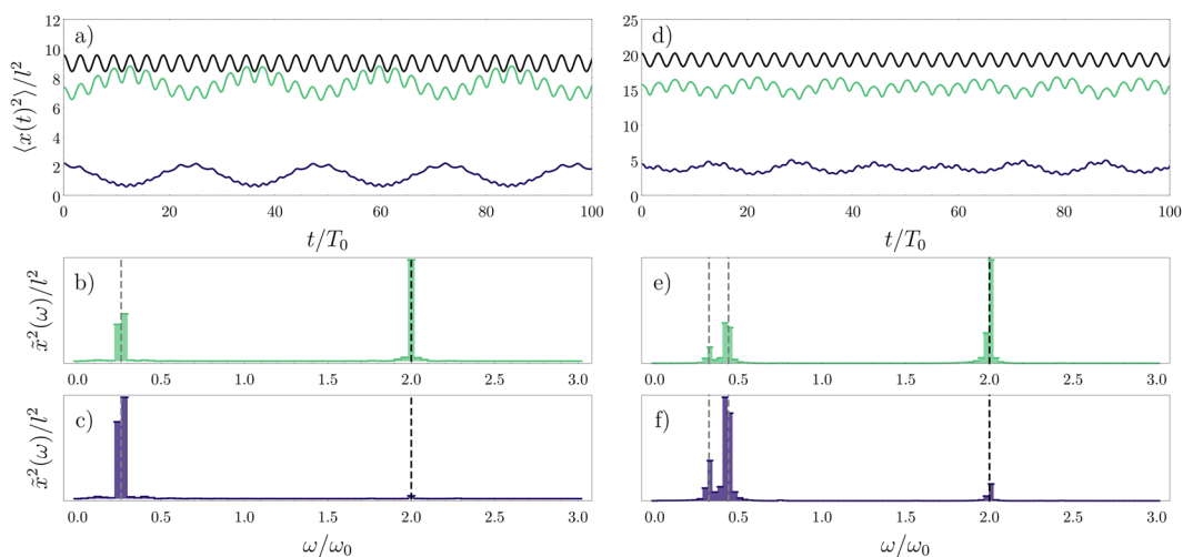
Figure 4. Dynamics in the SU(2) fermionic system for the (a–c) N = 4 ( 3 + 1 ) and (d–f) N = 6 ( 4 + 2 ) cases. In (a,d) we present the time evolution of the squared widths \langle x_c^2(t) \rangle (green) and \langle x_s^2(t) \rangle (blue) for each spin component, and \langle x_c^2(t) \rangle (black) for the total density. Panels (b,c,e,f) show the excitation peaks in the frequency domain, where the lower frequencies correspond to the spin dynamics. The black dashed lines mark the frequency of the total density oscillations ( \omega = 2\omega_0 ). The gray dashed lines correspond to gaps in the Floquet quasienergy spectrum of the time-dependent spin chain. In all cases, we assume g = 20 . This figure has been published, with modifications, in ref. 50 .
