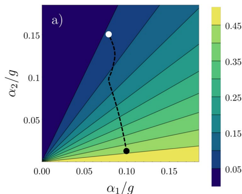
Figure 3. Numerical values of P_{\text{edge}} for different combinations of \alpha_1 and \alpha_2 . The black dashed curve corresponds to the trajectory of the exchange coefficients in time after the trap quench. The initial point is marked by the black dot, while the white dot marks the values of the exchange coefficients at t = T_0/2 . This figure has been published, with modifications, in ref. 50 .
