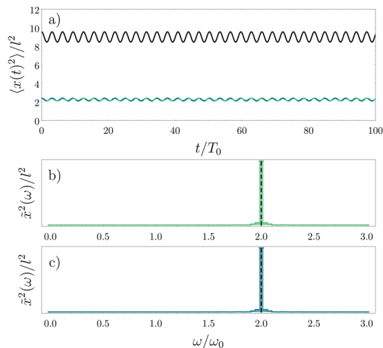
Figure 6. Dynamics in the SU(4) fermionic system. (a) Time evolution of the squared density widths \langle x_1^2(t) \rangle (green), \langle x_2^2(t) \rangle (dashed blue) and \langle x_c^2(t) \rangle (black). Panels (b,c) show the excitation peaks in the frequency domain for \langle x_1^2(t) \rangle and \langle x_2^2(t) \rangle , respectively. The black dashed lines mark the frequency of the total density oscillations. In these simulations, we assume g = 20 . This figure has been published, with modifications, in ref. 50 .
