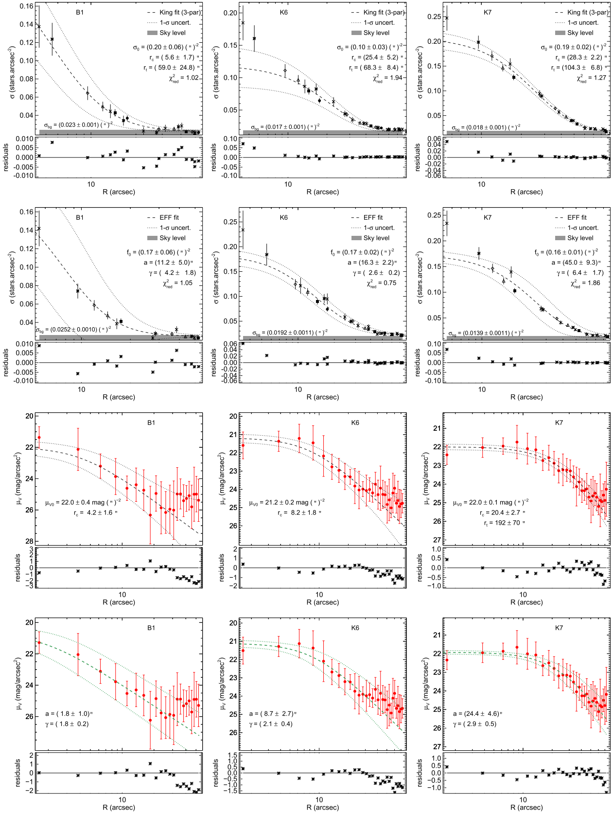
Figure 3. Radial density profiles for three SMC clusters and their respective King (first row) and EFF (second row) model fits (dashed line) with envelopes of 1 \sigma uncertainty (dotted lines). Different symbols correspond to the various widths of the annular bins employed. Surface brightness profiles for the same three SMC clusters and their respective King (third row) and EFF (fourth row) model fits (dashed line) and uncertainty (dotted lines). The best-fitting parameters are indicated and the fit residuals are plotted in the lower panels. The full set for the whole sample is published online.
