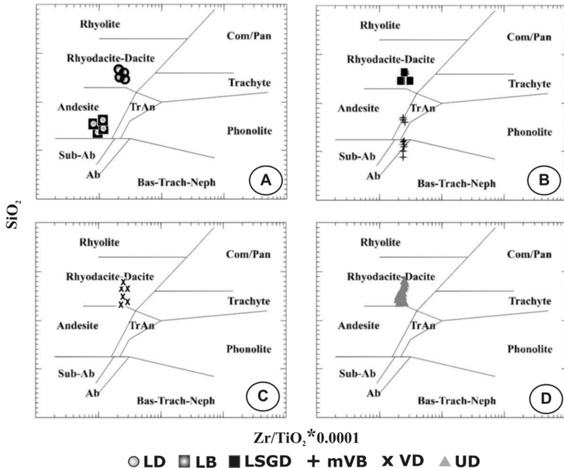
Figure 5 - Geochemical signature of the volcanic rocks of the Salto do Jacuí Mining District (Heemann, 1987). A) SiO 2 x Zr/TiO 2 diagram for the Lower Dacite and Lower Basalt units (R1 group); B) SiO 2 x Zr/TiO 2 diagram for the Lower Semi-glassy Dacite and mineralized Vesicular Basalt units; C) SiO 2 x Zr/TiO 2 diagram for the Vesicular Dacite unit; and D) SiO 2 x Zr/TiO 2 diagram for the Upper Dacite unit (R2A group).
