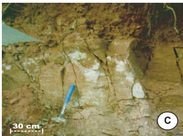
Figure 7 – Structural features of breccias related to Botucatu Fm. sandstone intertraps. A) Vesicular basalts fragments in sandstone matrix; B) Sandstone fragments in vesicular basalt matrix; C) Irregular Botucatu sandstone lens enclosed in vesicular basalt breccia.
