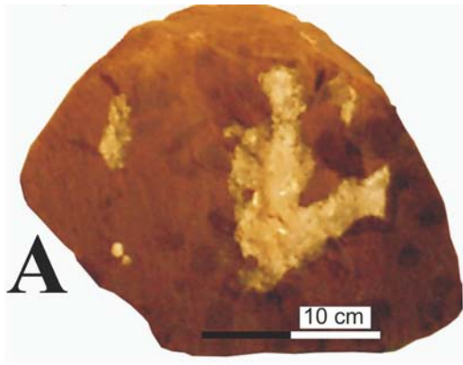
Figure 8 – Sandstone – volcanic rocks interaction structures in the Salto do Jacuí Mining District. A) Sandstone dyke cutting across Lower Semi-glassy Dacite; note, close to top right, a small lense of sandstone enclosed in the Lower Semi-glassy Dacite. B) Sandstone boulders (geodes) in the mineralized vesicular basalt (mVB); note thin sandstone sill like struture connecting sandstone geodes.
