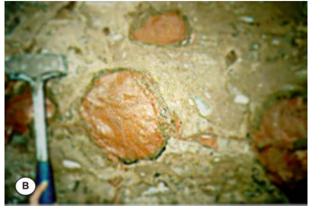
Figure 8 – Sandstone – volcanic rocks interaction structures in the Salto do Jacuí Mining District. A) Sandstone dyke cutting across Lower Semi-glassy Dacite; note, close to top right, a small lense of sandstone enclosed in the Lower Semi-glassy Dacite. B) Sandstone boulders (geodes) in the mineralized vesicular basalt (mVB); note thin sandstone sill like struture connecting sandstone geodes.
