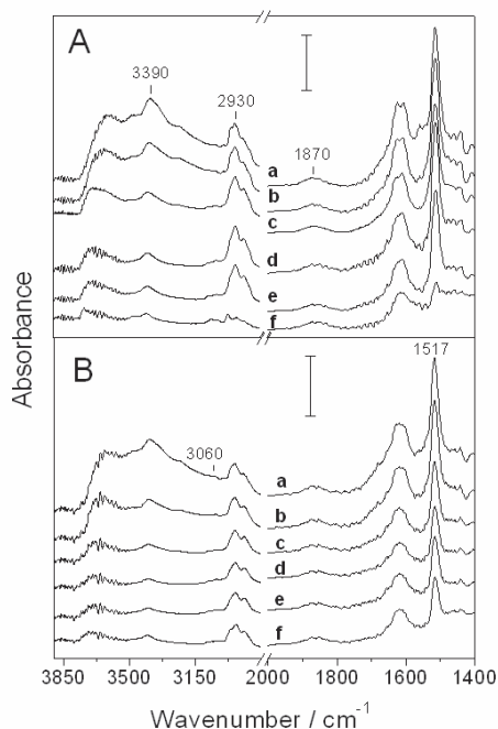
Figure 1: FTIR absorbance spectra for xerogel samples A and B, obtained at room temperature, after heating in vacuum, for 1 hours at: a) 100, b) 200, c) 300, d) 350, e) 400 and f) 450 °C. The bar value is 0.2 for both samples.
