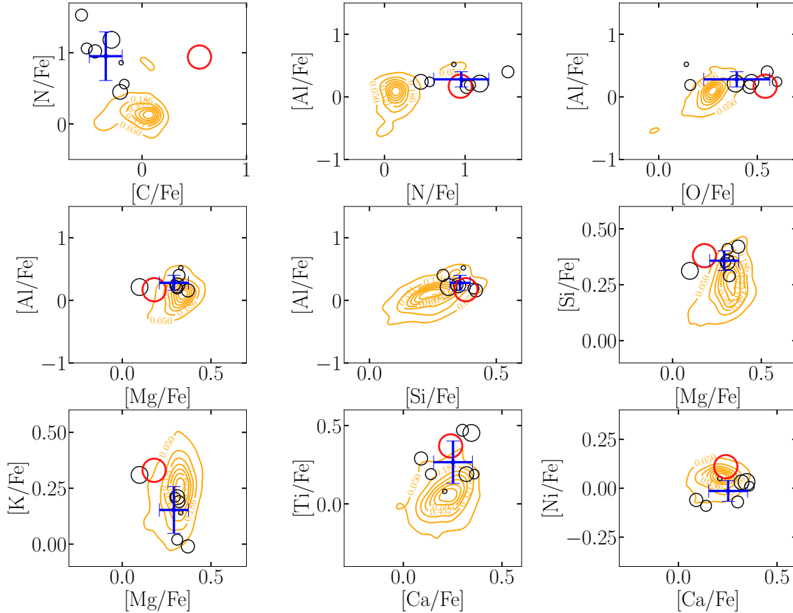
Fig. 4. Distributions of various elemental-abundance ratios from the APOGEE-2 survey for bulge field stars in close proximity to the Galactic Centre ( -20^\circ < l < 20^\circ and |b| < 20^\circ ), and comparison with stars in NGC 6723. The field-star abundances are represented by orange iso-abundance contours. The member stars of NGC 6723 and the extra-tidal star analyzed in this work are shown with black and red open circles, respectively. The circle sizes reflect their V_o magnitudes, with decreasing size for fainter magnitudes. The blue cross symbol denotes the average ( \langle [X_i/Fe] \rangle ) and its associated star-to-star scatter ( \sigma_{([X_i/Fe])} ) of the abundance derived from the seven member NGC 6723 stars analyzed in this work.
