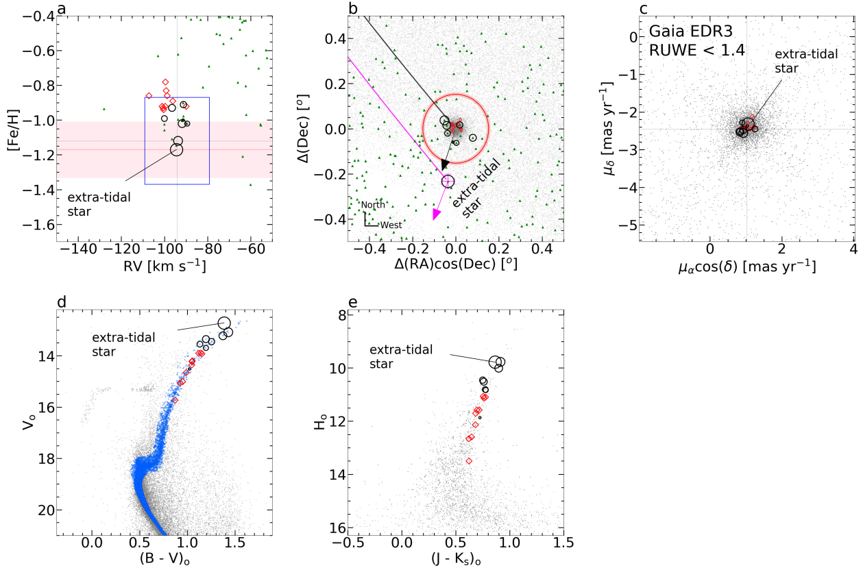
Fig. 1. Properties of the extra-tidal star compared with likely members of NGC 6723. Panel a: metallicity – radial velocity plane for stars in the APOGEE-2 catalogue in the region of NGC 6723 (green triangles). The black open circles are potential members of NGC 6723; sizes reflect their V_o magnitudes, with decreasing size for fainter magnitudes. The pink line and shaded region indicate the ([Fe/H]) \pm \sigma_{[Fe/H]} of the extra-tidal star. The black dotted lines indicate the nominal [Fe/H] and radial velocity of NGC 6723 from Harris (1996, 2010). The red unfilled diamonds refer to probable members analysed in the literature (Crestani et al. 2019). The blue rectangle indicates the region adopted to choose potential cluster members, based on radial velocity and metallicity (see Sect. 2). Panel b: positions for stars in the APOGEE-2 and Gaia EDR3 (grey dots) catalogues in the region of NGC 6723. The magenta cross symbol indicates the Gaia astrometric uncertainty. The big red and shadow circumference show the cluster tidal radius ( r_t = 9.14 \pm 0.49' ) of NGC 6723 determined in this work from HST + Gaia EDR3 data set (see Sect. 8). The orbital paths of the cluster (black line) and the extra-tidal star (magenta line) are shown, along with the proper motion vectors (black arrow) of the cluster from Baumgardt et al. (2019), and the extra-tidal star (magenta arrow); their lengths (scaled up for visibility) and directions are essentially identical. Panel c: proper-motion plane for the selected candidates. Panels d and e: V_o versus (B - V)_o and 2MASS H_o versus (J - K_s)_o Colour-Magnitude Diagram (CMD) centred on NGC 6723, showing all the stars within the cluster tidal radius, and the probable cluster members (cyan symbols) within a 2\sigma deviation from the best isochrone fitting (Souza et al. 2020; Oliveira et al. 2020). The largest open circle in all panels indicate the extra-tidal star.
