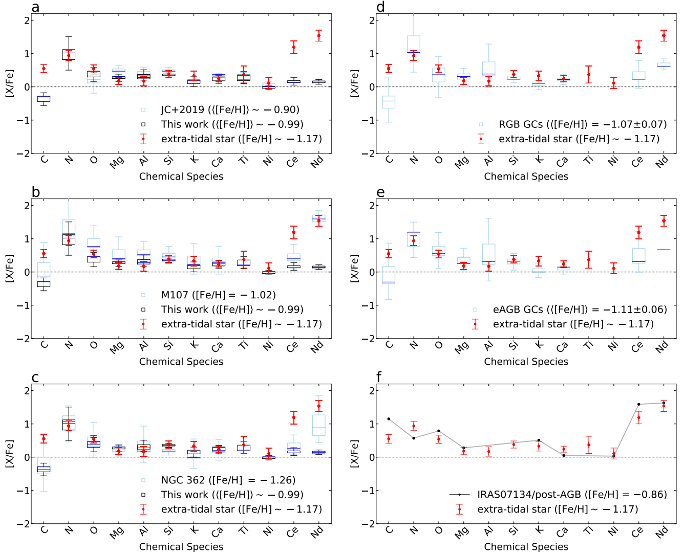
Fig. 3. Comparison of elemental-abundance ratios of likely member stars for NGC 6723 with other GCs of similar metallicity, and the extra-tidal star with RGB and early-AGB (eAGB) cluster stars, and IRAS07134 star. Panel a: elemental-abundance patterns for our sample (black boxes and red dot) compared to the spectroscopic study of NGC 6723 Crestani et al. (2019) ; (light blue boxplots). Panel b: comparison with M 107 ( Mészáros et al. 2020 ). Panel c: comparison with NGC 362 ( Mészáros et al. 2020 ). Panel d: elemental-abundance patterns for the extra-tidal star compared to those of RGB GC stars. Panel e: compared with early-AGB GC stars ( Mészáros et al. 2020 ). Panel f: comparison with a field post-AGB star, IRAS 07134 ( De Smedt et al. 2016 ), with comparable atmospheric parameters. Boxes represent the inter-quartile ranges (IQR), whiskers the 1.5 \times \text{IQR} limits, and blue lines the medians.
