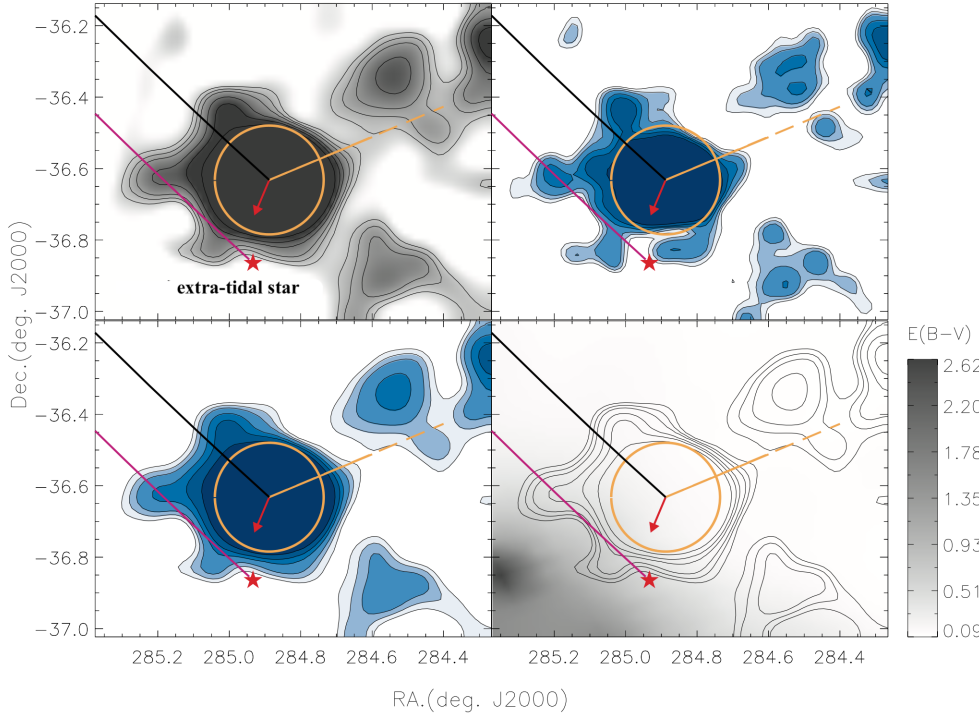
Fig. 7. Modified Fig. 10 from Chun et al. (2015). The red ‘star’ symbol shows the position of the newly identified extra-tidal star. The orange circle indicates the cluster tidal radius ( r_t = 9.14 \pm 0.49' , see Sect. 8), and the red arrow defines the proper motion of NGC 6723 from Baumgardt et al. (2019). The orange solid and dashed line shows the direction of the Galactic Centre and Galactic plane, respectively. Top-left panel: star-count map around the cluster; the top-right panel is the surface-density map, smoothed by a Gaussian kernel 0.07^\circ ; the lower-left panel is the same data, but smoothed with a 0.11^\circ kernel; the bottom-right panel shows the distribution map of E(B-V) . The iso-density contour levels shown are 2.0\sigma , 2.5\sigma , 3.0\sigma , 4.0\sigma , 5.0\sigma , and 7.0\sigma . The orbital path of the cluster (black line) and the extra-tidal star (purple line) is over-plotted.
