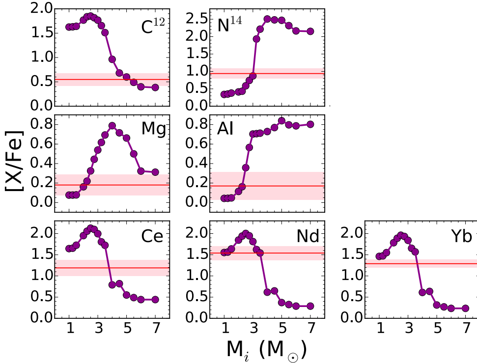
Fig. 5. Predicted abundance ratios, as a function of the initial stellar mass, for low-and-intermediate-mass stars. [X_i/Fe] values were obtained from stellar yields by Karakas et al. (2014, 2018). For comparison, the red line and shaded red bands represent the observed abundance ratios and sensitivities for our extra-tidal star.
