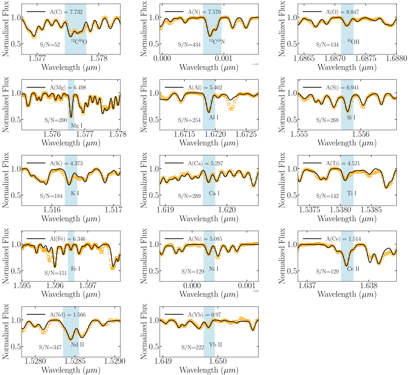
Fig. 2. High-resolution near-IR H -band spectrum of the extra-tidal star. The spectral regions are shown with orange squares. Superimposed is the best-fit of a MARCS/BACCHUS spectral synthesis (black line). The light blue shaded regions show the strength of the molecules ( ^{12}\text{C}^{16}\text{O} , ^{12}\text{C}^{14}\text{N} , ^{16}\text{OH} ), and the atomic lines, namely the \alpha -elements (Mg I, Si I, Ca I, Ti I), the odd- Z elements (Al I, K I), the iron-peak elements (Fe I, Ni I), and the s -process elements (Ce II, Nd II, Yb II), expressed in air wavelengths. The legends in each panel show the absolute abundance, A(X) , of the species under consideration, and the signal-to-noise (S/N) in the regions of the features, respectively.
