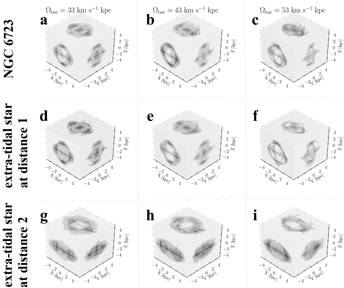
Fig. 6. Thousand-orbit realisations of NGC 6723 and the extra-tidal star time-integrated for 2 Gyr. The dark colours correspond to the most probable regions of the space, which are crossed more frequently by the simulated orbits, assuming three different values of the angular velocity of the bar ( \Omega_{\text{bar}} = 33, 43, \text{ and } 53 \text{ km s}^{-1} \text{ kpc} ). Panels a–c: orbits of NGC 6723, using as initial conditions the observed values from Baumgardt et al. (2019) ; the middle and bottom rows show the orbits of the extra-tidal star, adopting the observed values from the Table 1 , and an assumed heliocentric distance at 8.3 kpc ( panels d–f ), and 6.24 kpc ( panels g–i ).
