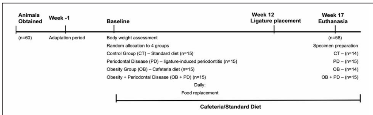
Fig. 1: Study Flowchart.
