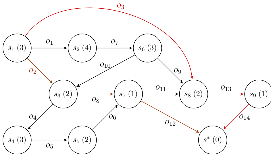
Figure 3.2 – Example sample set graph with two shortest paths (red, orange) from s_1 to the goal s^* . The h -value of each state is in parenthesis.
