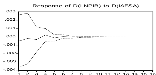
Response to Generalized One S.D. Innovations \pm 2 S.E.
