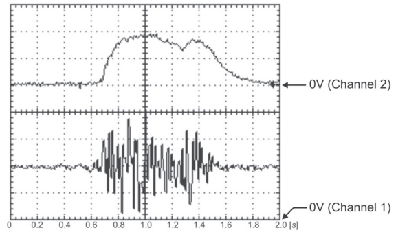
Figure 4. RMS value (Channel 2: 500 mV/div) and Biceps muscle signal (Channel 1: 1 V/div).
