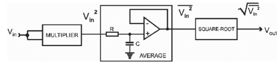
Figure 3. Classic topology for generation of RMS value using analog circuits.
