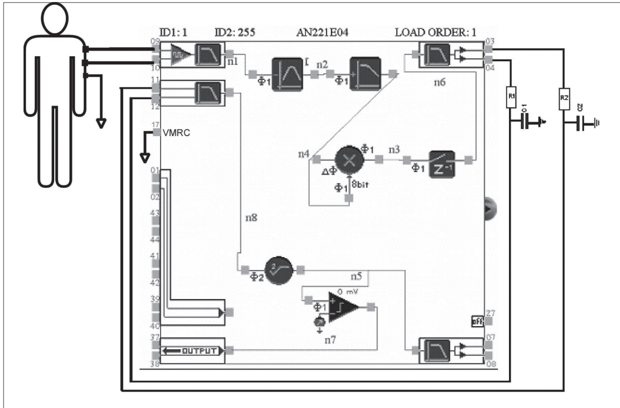
Figure 5. Complete FPAACircuit for acquisition of EMG signal.
