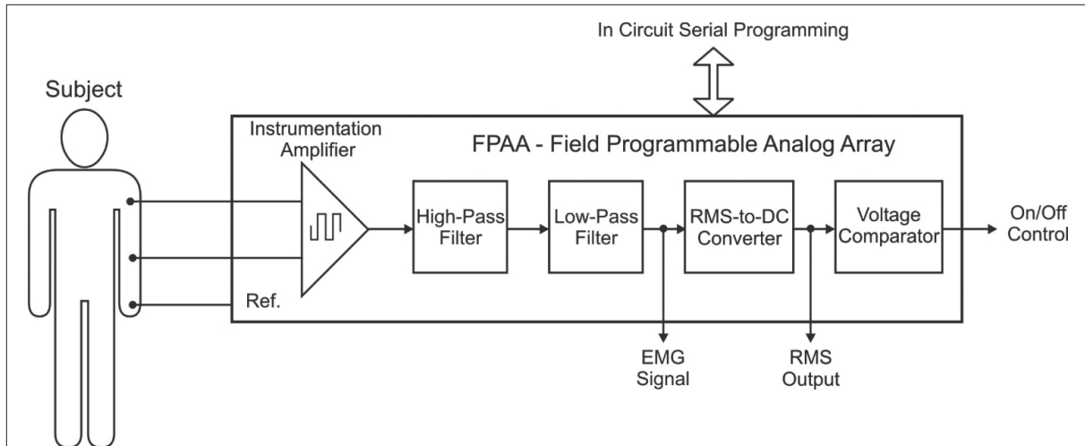
Figure 1. Block diagram of the proposed system for EMG signal acquisition and processing.
