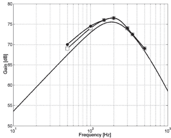
Figure 2. Frequency response plots: Matlab® simulations (solid line), AnadigmDesigner@2 simulation (□) and experimental (●).
