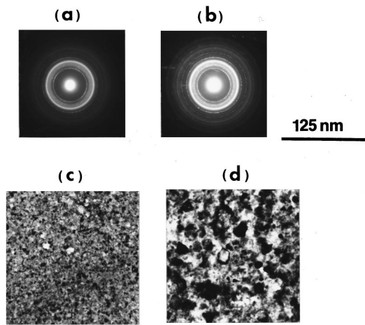
FIG. 4. Bright-field micrographs and diffraction patterns showing a typical in situ recrystallization sequence: (a)(b) diffraction patterns after post-irradiation annealing for 1200 and 1500 s at 973 K, showing that recrystallization has taken place, with the formation of crystalline intermetallic compounds (c)(d) corresponding bright-field micrographs after 20 and 25 minutes of annealing, showing the change in contrast associated with the growth of grains of crystalline intermetallic compounds.
