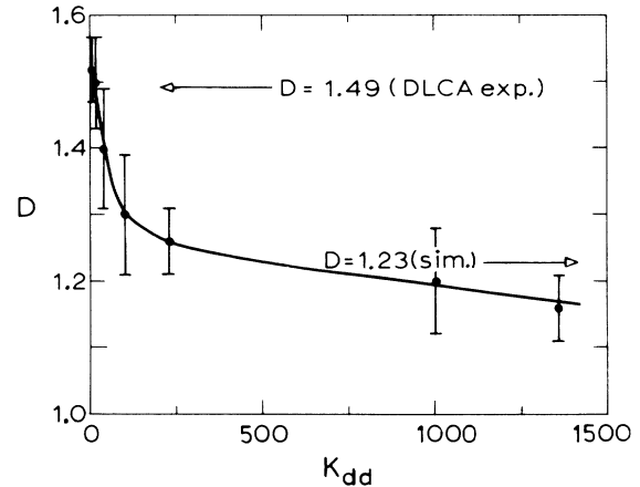
FIG. 2. Fractal dimension D vs dipolar coupling constant K_{dd} . The value D=1.49\pm 0.06 for K_{dd}\rightarrow 0 was found in earlier aggregation experiments (Ref. 1) for nonmagnetic spheres. It is also seen that for large K_{dd} , D approaches the simulated value D=1.23\pm 0.12 as discussed in the text. The solid line is only a guide to the eye.
