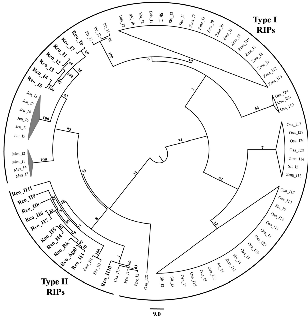
Figure S1 - Maximum likelihood phylogenetic tree showing the evolutionary relationships among the Brachypodium distachyo (Bdi), Cucumis sativus (Csa), Jatropha curcas (Jcu), Manihot esculenta (Mes), Oryza sativa (Osa), Populus trichocarpa (Ptr), Prunus persica (Ppe), R. communis (Rco), Setaria italic (Sit), Sorghum bicolor (Sbi) and Zea mays (Zma) RIPs. The primary clustered monocot RIPs are shown as white sectors, the RIPs corresponding to a Euphorbiaceae clade are indicated as gray sectors and the RIPs from R. communis clades are indicated in bold characters. The midpoint root and bootstrap values are also indicated.
