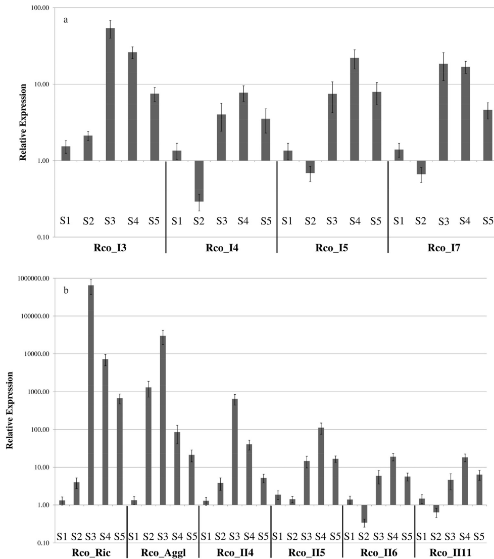
Figure 6 - Relative gene expression of R. communis RIPs as measured by RT-qPCR in the five stages of seed development. (A) The relative expression levels of Rco_I3, 4, 5 and 7. (B) The relative expression levels of Rco_Ric, Rco_Aggl and Rco_II 4, 5, 6 and 11. The expression data are shown on a logarithmic scale. The RIP gene expression levels were normalized at the S1 stage by the 2^{-\Delta\Delta Ct} method using the elongation factor B (29785.m000934), ubiquitin (30169.m006323) and ubiquitin conjugation protein rad6 (29736.m002026) genes. The bars represent the mean \pm standard deviations ( n = 4 ).
